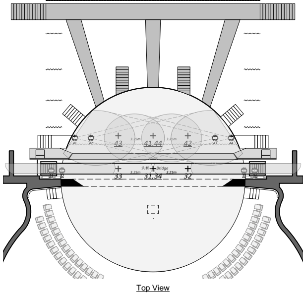
FOH 5 - Claypaky Scenius Profile
